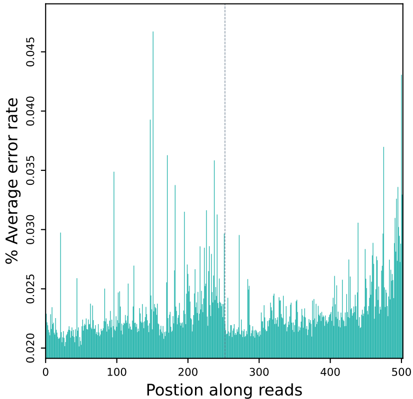
Error rate distribution along reads (R20115)
